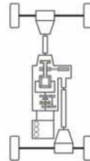
Neutral: Central differential unlocked. No power is sent to any wheel. Switch to this mode in the rare event of your vehicle being towed.
