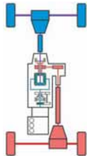
4 High: Central differential on. Power is sent to all wheels, all the time. Switch to this mode for normal driving.
