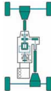
4 High Lock: Central differential locked. Power sent to front and rear wheels equally. Switch to this mode for medium off roading.
