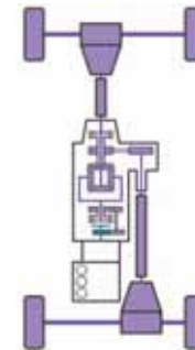
4 Low Lock: Central differential locked. Power sent to front and rear wheels equally but after increasing the torque using a 'traction enhancer'. Switch to this mode when stuck in mud, sand or snow.
